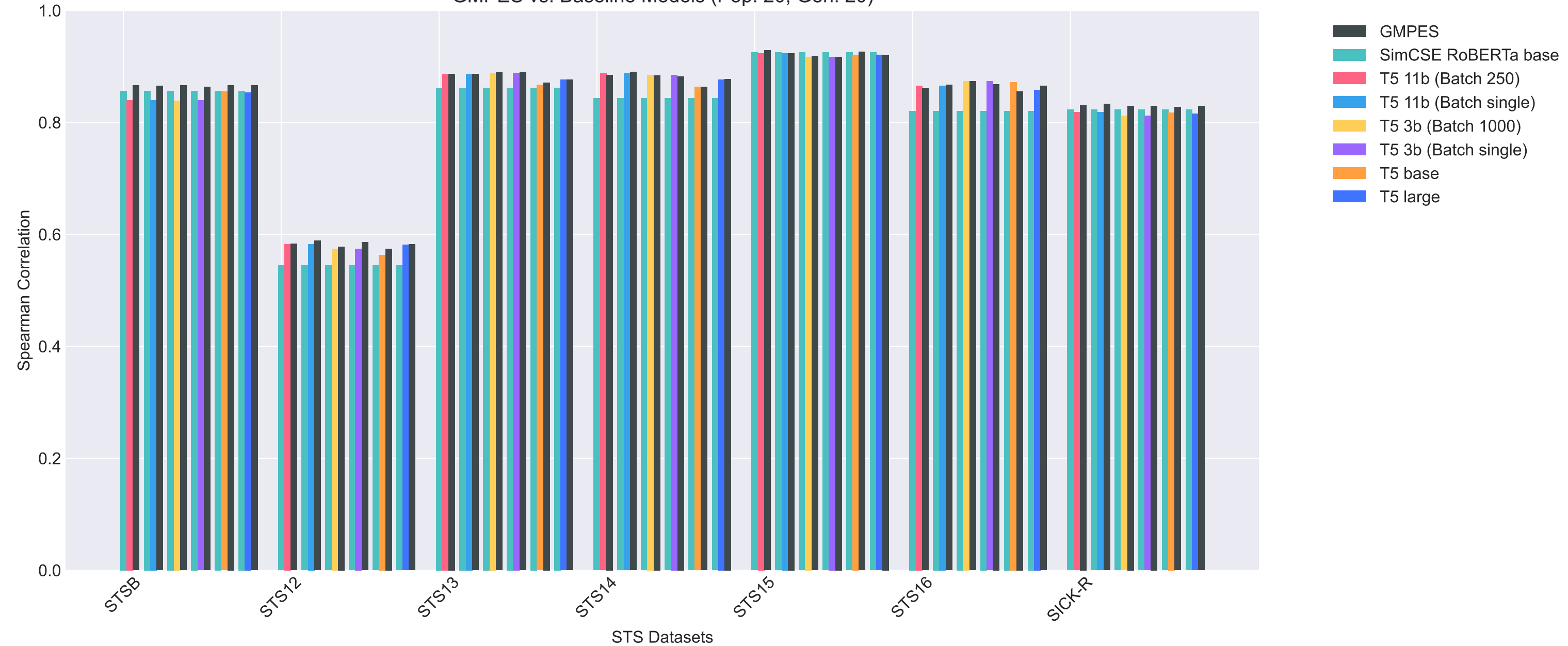
GMPES vs. Baseline Models (Pop: 20, Gen: 20)
